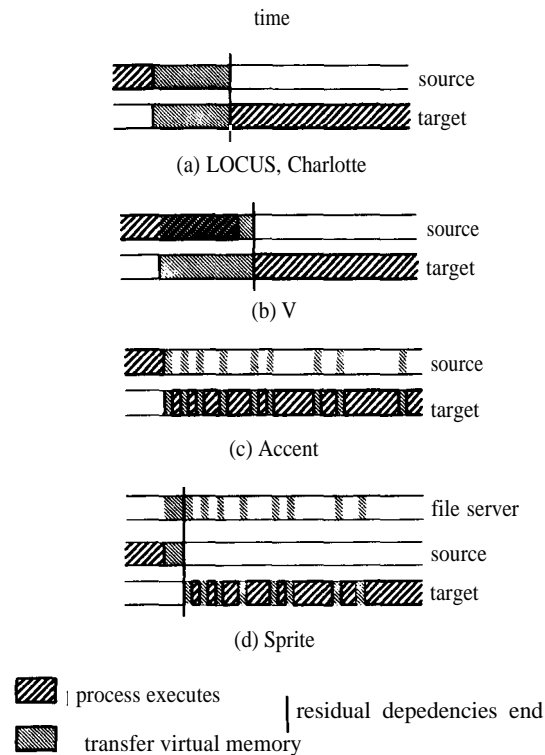
Figure 1. Different techniques for transferring virtual memory. (a) shows the scheme used in LOCUS and Charlotte, where the entire address space is copied at the time a process migrates. (b) shows the pre-copying scheme used in V, where the virtual memory is transferred during migration but the process continues to execute during most of the transfer. (c) shows Accent's lazy-copying approach, where pages are retrieved from the source machine as they are referenced on the target. Residual dependencies in Accent can last for the life of the migrated process. (d) shows Sprite's approach, where dirty pages are flushed to a file server during migration and the target retrieves pages from the file server as they are referenced. In the case of eviction, there are no residual dependencies on the source after migration. When a process migrates away from its home machine, it has residual dependencies on its home machine throughout its lifetime
