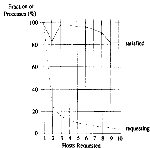
Figure 7. Distribution of host requests and satisfaction rates. For a given number of hosts, shown on the X-axis, the line labelled 'requesting' shows the fraction of processes that requested at least that many hosts. The line labelled 'satisfied' shows, out of those processes that requested at least that number of hosts, the fraction of processes that successfully obtained that many hosts. Thus, 98 per cent of all processes were able to obtain at least one host, and over 80 per cent of processes that requested at least ten hosts obtained 10 hosts. Only 24 per cent of processes requested more than one host
