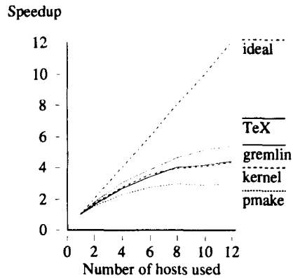
Figure 5. Speed-up of compilations using a variable number of hosts. This graph shows the speed-up relative to running pmake on one host (i.e. without migration). The speed-up obtained depends on the extent that hosts can be kept busy, the amount of parallelization available to pmake and system bottlenecks
