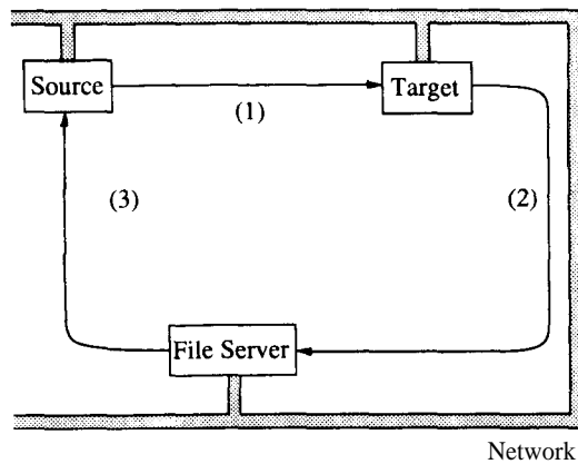
Figure 2. Transferring open files. (1) The source passes information about all open files to the target; (2) for each file, the target notifies the server that the open file has been moved; (3) during this call the server communicates again with the source to release its state associated with the file and to obtain the most recent state associated with the file
