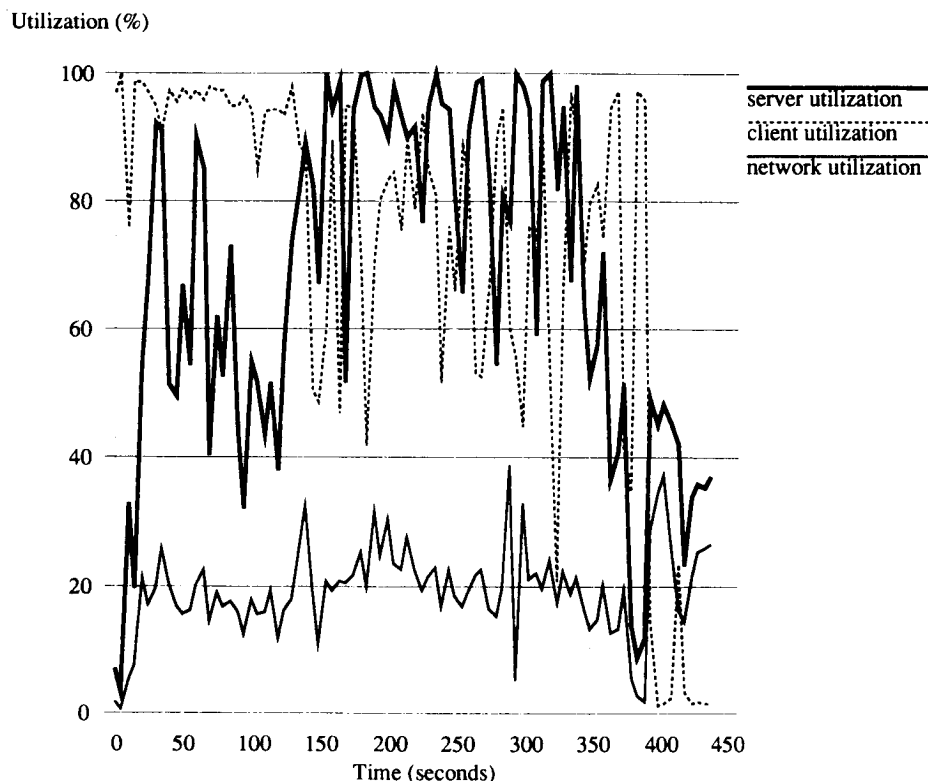
Figure 6. Processor and network utilization during the 12-way pmake. Both the file server and the client workstation running pmake were saturated
