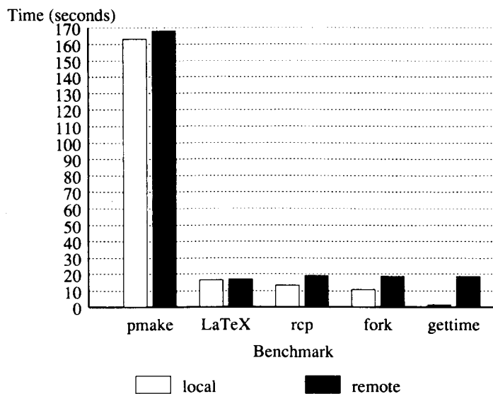
Figure 3. Comparison between local and remote execution of programs. The elapsed time to execute CPU-intensive and file-intensive applications such as pmake and LATEX showed negligible effects from remote execution (3 and 1 per cent degradation, respectively). Other applications suffered performance penalties ranging from 42 per cent (rcp), to 73 per cent (fork), to 3200 per cent (gettime)
