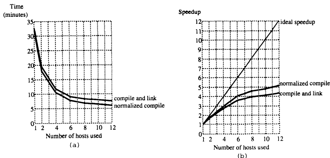
Figure 4. Performance of recompiling the Sprite kernel using a varying number of hosts and the pmake program. Graph (a) shows the time to compile all the input files and then link the resulting object files into a single file. In addition, it shows a 'normalized' curve that shows the time taken for the compilation only, deducting as well the pmake start-up overhead of 19 s to determine dependencies; this curve represents the parallelizable portion of the pmake benchmark. Graph (b) shows the speed-up obtained for each point in (a), which is the ratio between the time taken on a single host and the time using multiple hosts in parallel
