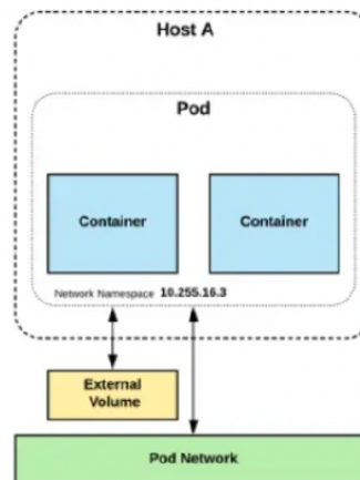
Figure 11.2: Visualization of the relationship between containers, pods, and hosts.
