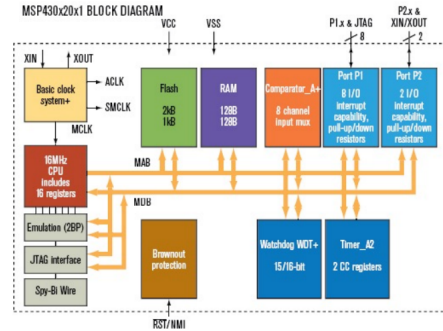
Figure 27.1: MSP430 board
