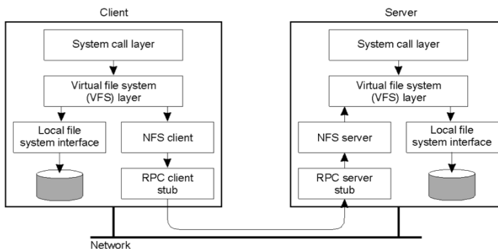
Figure 23.3: Network File System (NFS)
