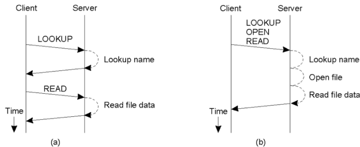
Figure 23.4: Difference in communication in NFS version 3 and version4.
