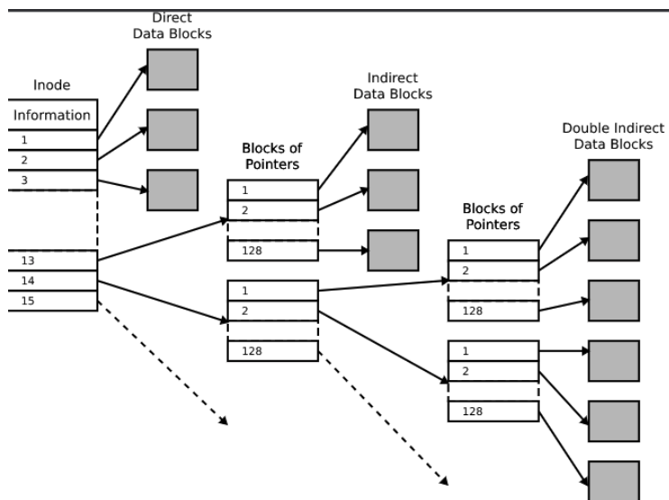
Figure 23.1: Inode structure
