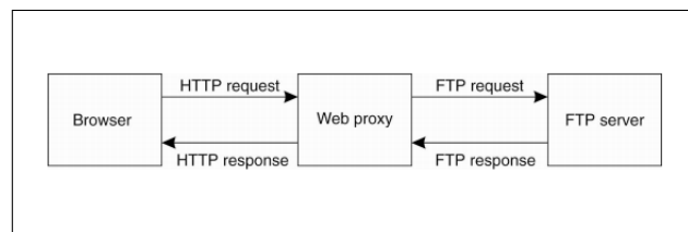
Figure 21.4: Web Proxy
