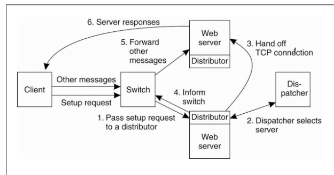
Figure 21.7: Scalable Content-Aware Cluster of Web servers
