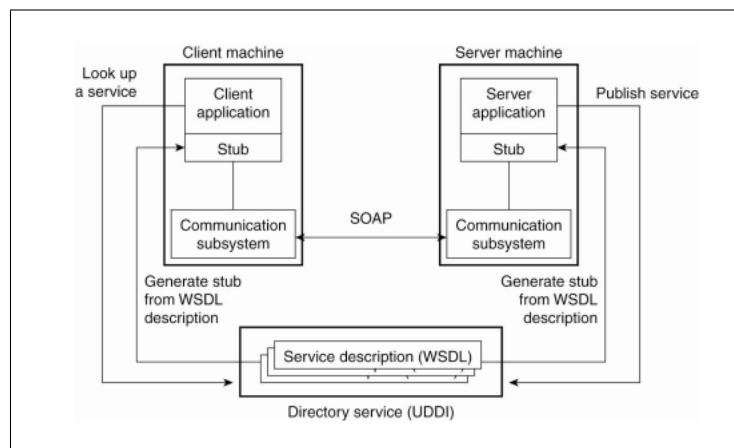
Figure 21.12: Web service
