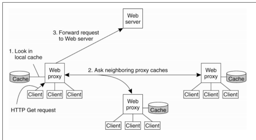
Figure 21.15: Cooperative Caching
