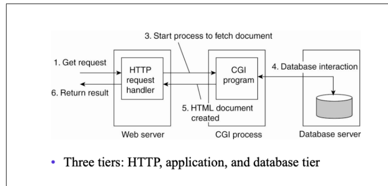
Figure 21.5: Multitiered architecture
