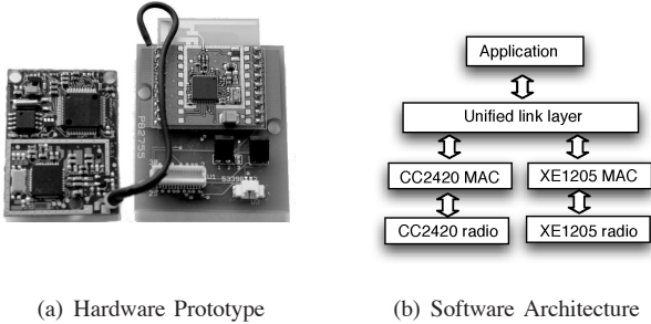
Fig. 3. System Components: (a) Hardware prototype comprising the Tinynode and a CC2420 expansion board and (b) Unified Link Layer for the radios
