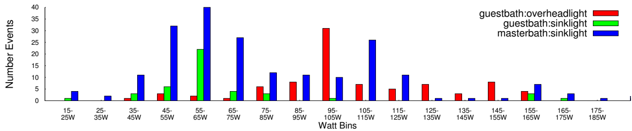
Fig. 7. Histogram of events for each 10W power bin for selected switches using the reactive learning technique.
