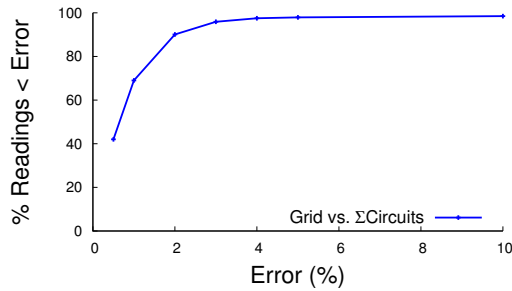
Fig. 4. Error between our deployment home’s aggregate electricity data and the sum of all the individual circuits
