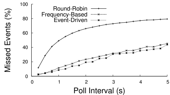
Fig. 9. Frequency- and event-driven polling capture more energy events than basic round-robin polling.
