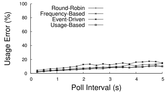
Fig. 8. Even low-frequency polling results in accurate per-device energy usage information.
