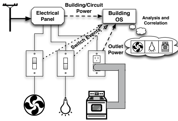
Fig. 1. Our monitoring and control architecture.
