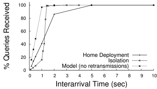
Fig. 2. Insteon does not support high outlet query rates.
