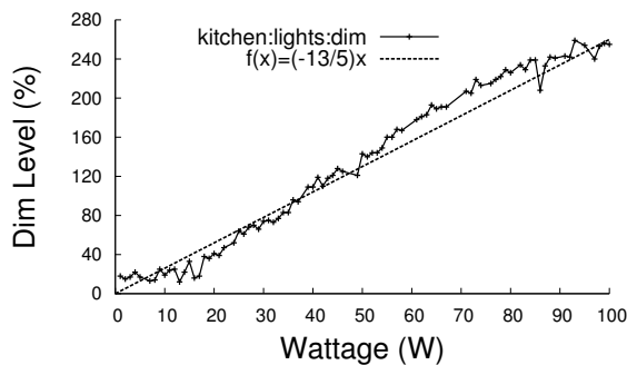
Fig. 6. Power usage is a linear function of a light’s dim level.
