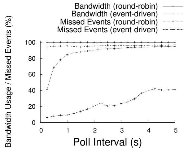
Fig. 11. Event-driven polling effectively utilizes bandwidth to monitor highly variable devices.
