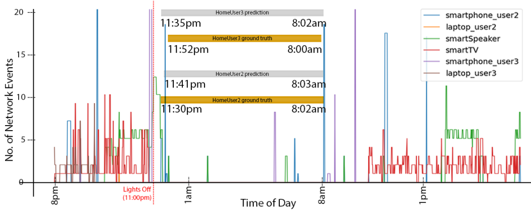
Fig. 23. Model performance on device usage for HomeUser 2 and HomeUser 3 .
