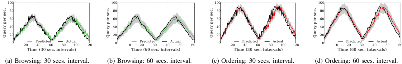
Figure 4. Comparison of regression-based model predicted rates with empirical measurements. Predicted and actual query rates over time for the browsing and ordering workload mixes. The shaded areas represent the 95 th percentile confidence interval. For both workload types, the prediction accuracy is higher for a larger prediction window.
