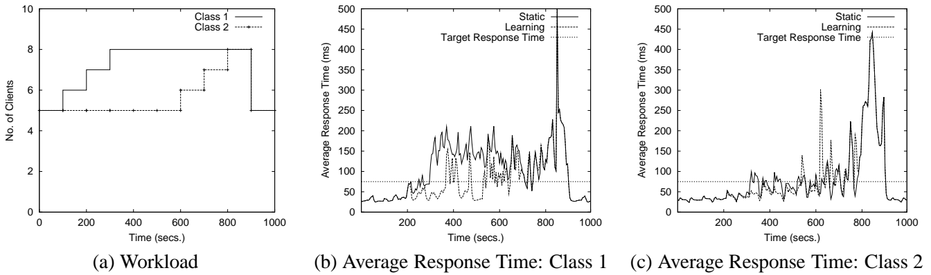
Figure 4: Behavior of the learning-based dynamic bandwidth allocation technique.
