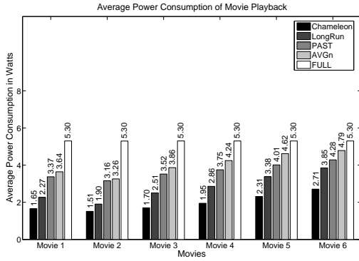
(a) Average CPU Power Consumption
