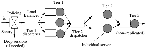
Figure 2. Architecture of a 3-tier Internet Application. In this example, tiers 1 and 2 are clustered, while tier 3 is not.
